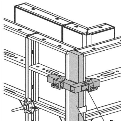
Pince angle
