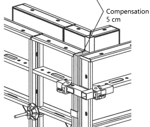
Pince angle
