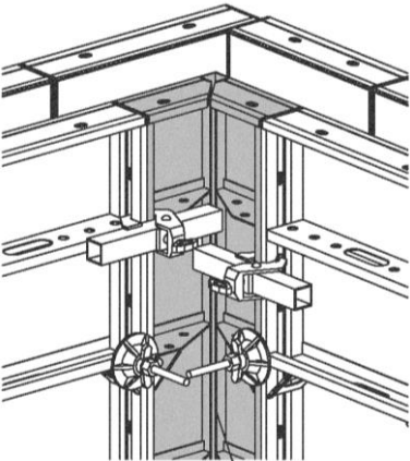
Internal corner 300
